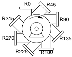
Discharge positions viewed from drive end-right hand
