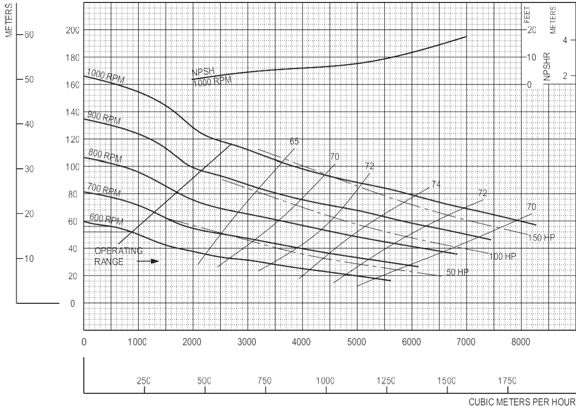
12NHPP - VARIOUS RPM
